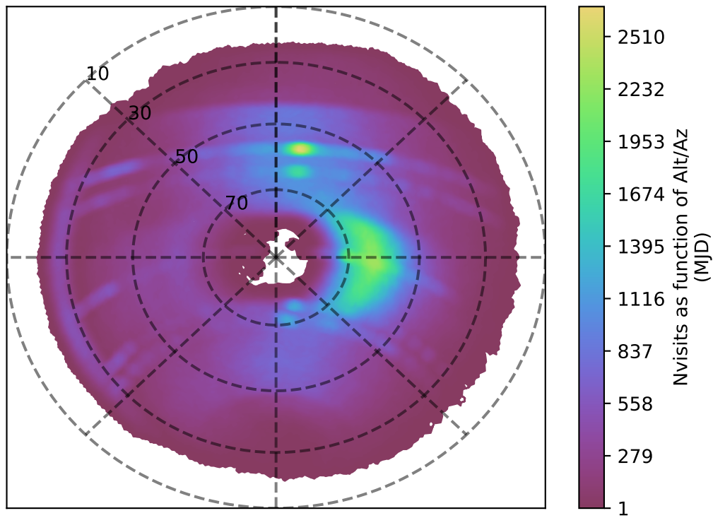
too_elab_r16_d2_griz_v3.4_10yrs r band: Nvisits as function of Alt/Az
