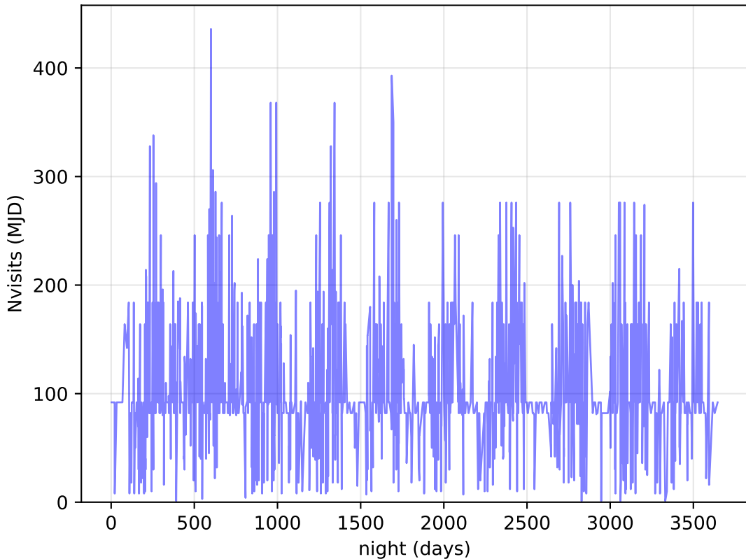
too_elab_r16_d2_griz_v3.4_10yrs DDF: Nvisits
