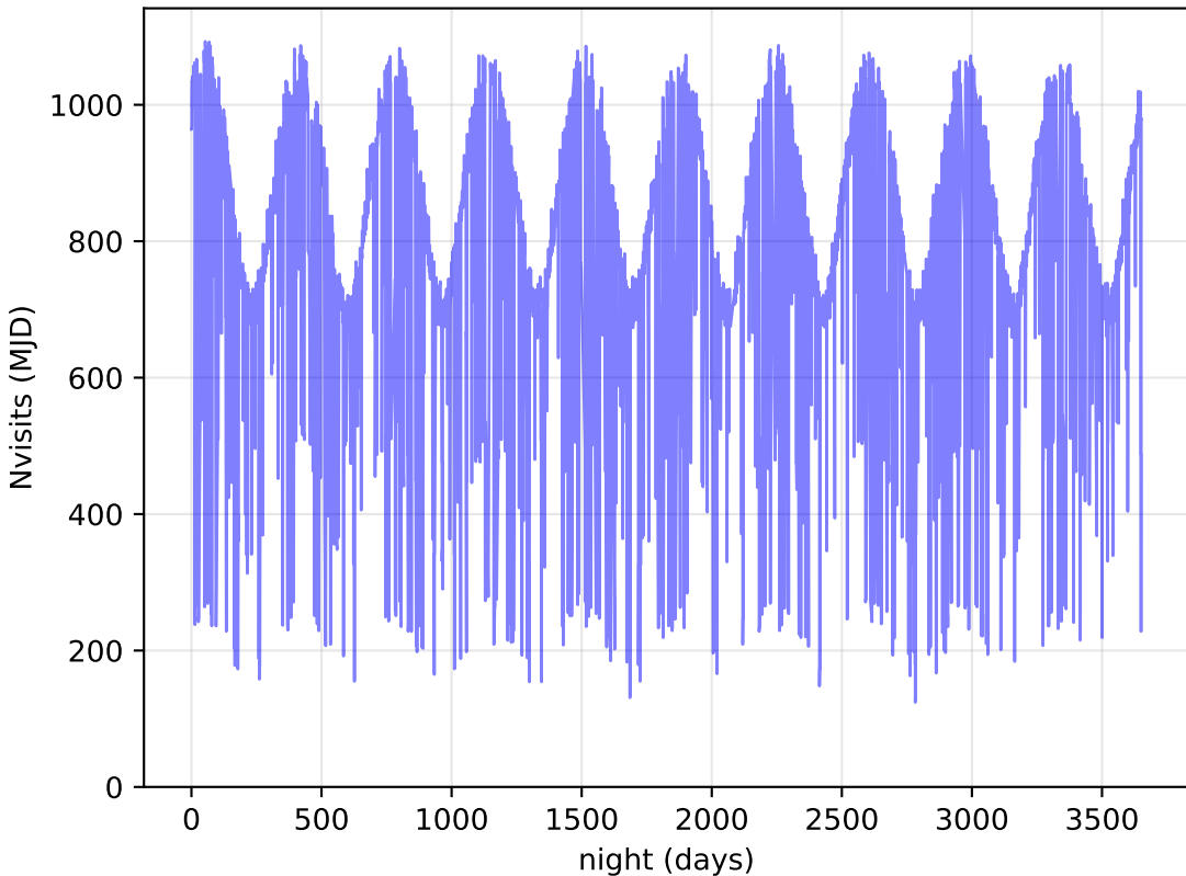
too_elab_r16_d2_griz_v3.4_10yrs All visits: Nvisits
