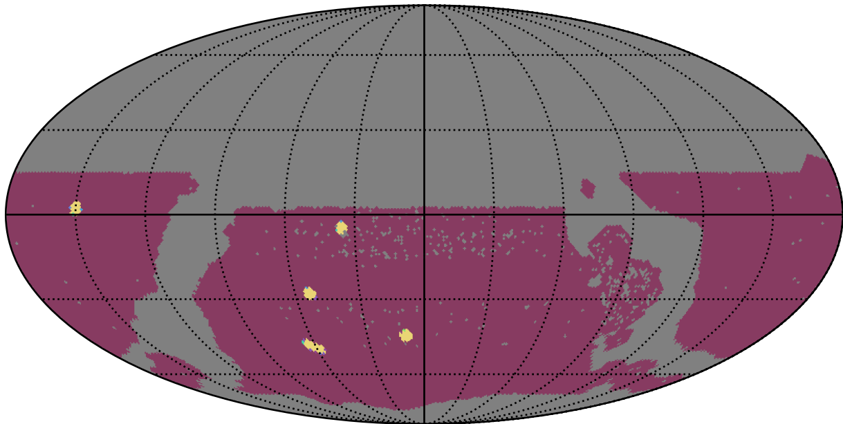
too_elab_r16_d2_griz_v3.4_10yrs WFD: NumberOfQuickRevisits
