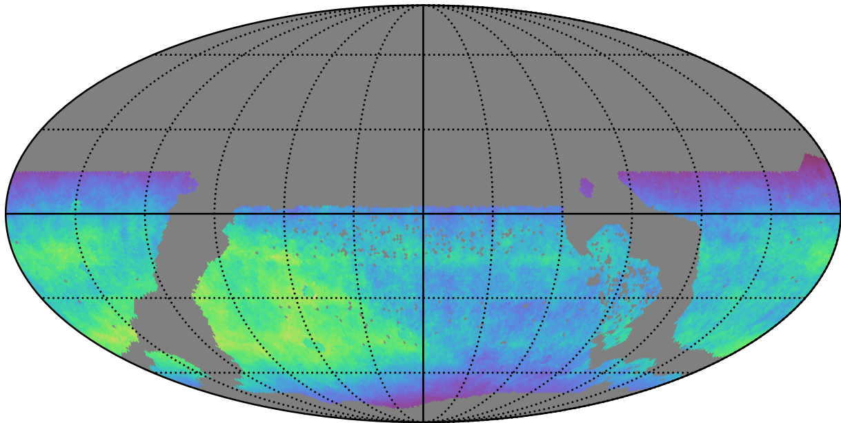
too_elab_r16_d2_griz_v3.4_10yrs WFD z band: Normalized Teff
