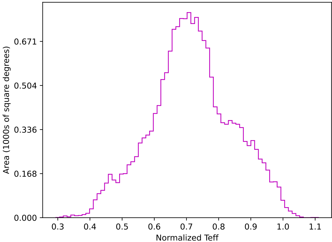
too_elab_r16_d2_griz_v3.4_10yrs WFD z band: Normalized Teff
