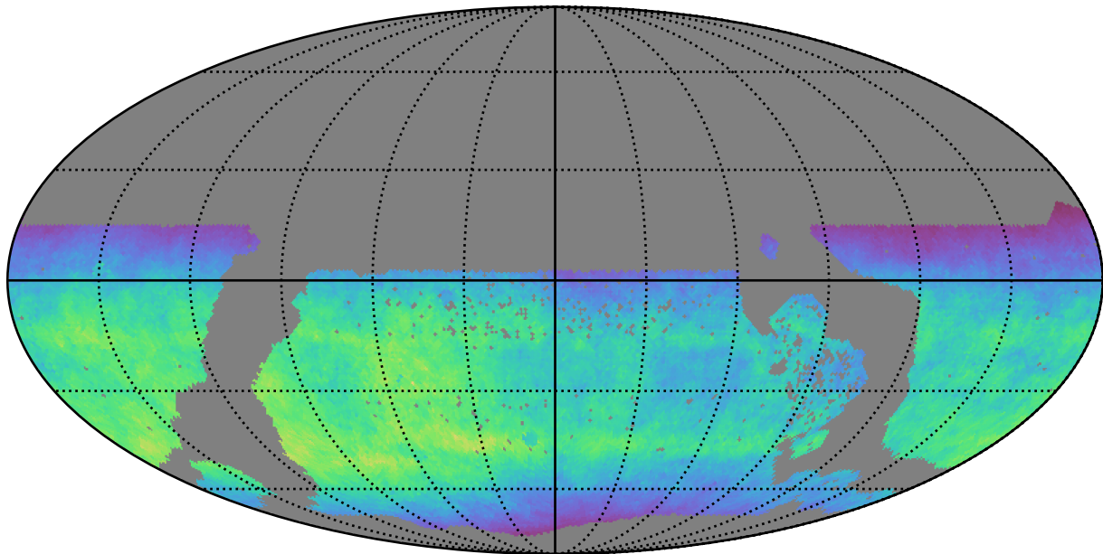
too_elab_r16_d2_griz_v3.4_10yrs WFD y band: Normalized Teff
