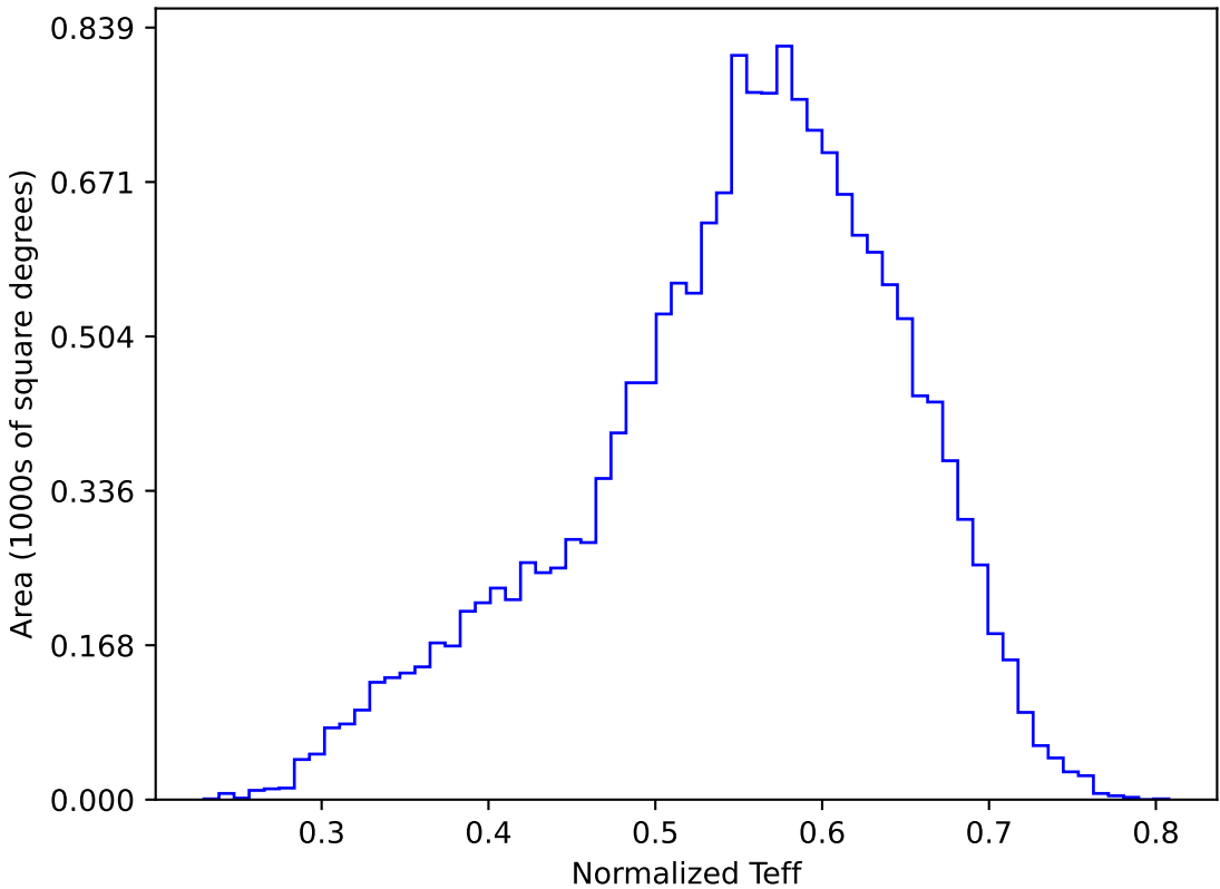
too_elab_r16_d2_griz_v3.4_10yrs WFD y band: Normalized Teff
