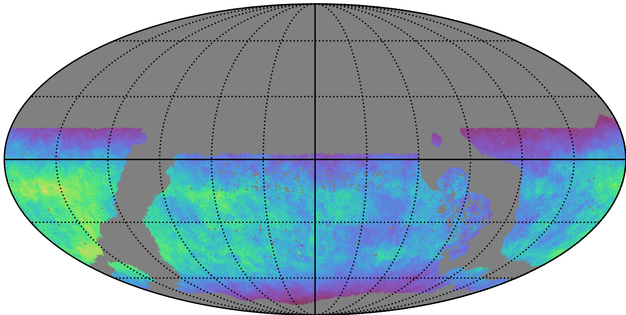
too_elab_r16_d2_griz_v3.4_10yrs WFD u band: Normalized Teff
