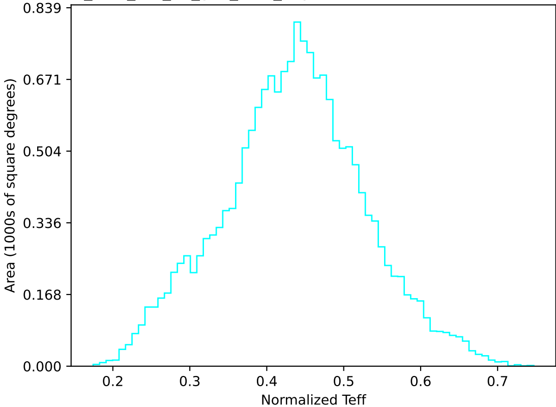
too_elab_r16_d2_griz_v3.4_10yrs WFD u band: Normalized Teff
