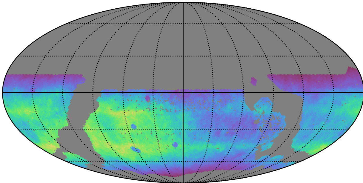
too_elab_r16_d2_griz_v3.4_10yrs WFD r band: Normalized Teff
