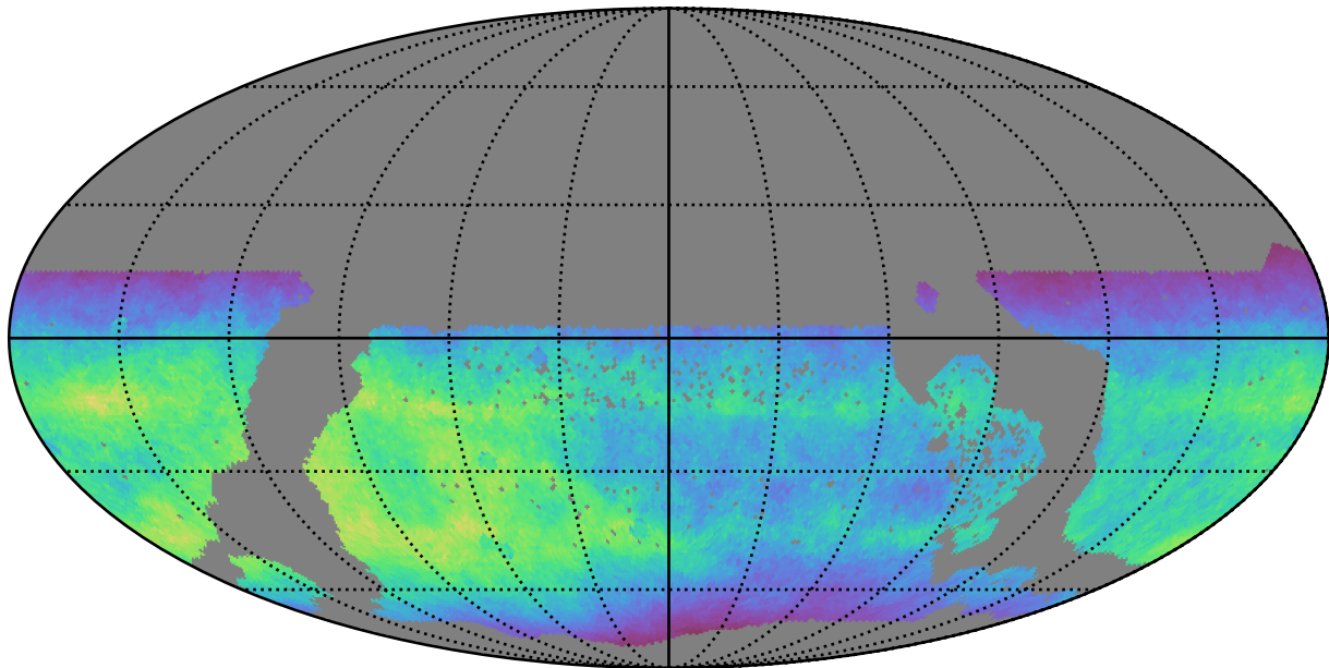
too_elab_r16_d2_griz_v3.4_10yrs WFD i band: Normalized Teff
