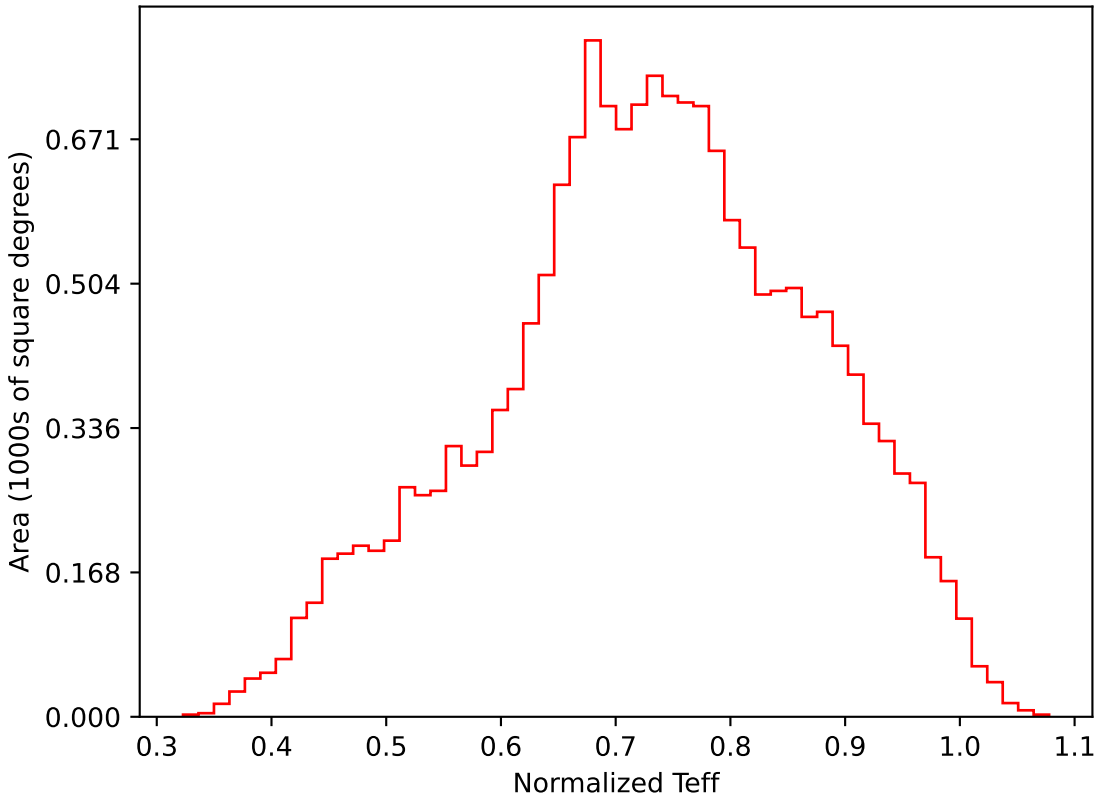
too_elab_r16_d2_griz_v3.4_10yrs WFD i band: Normalized Teff
