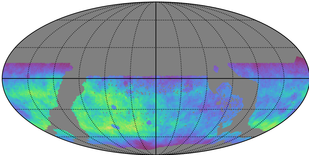
too_elab_r16_d2_griz_v3.4_10yrs WFD g band: Normalized Teff
