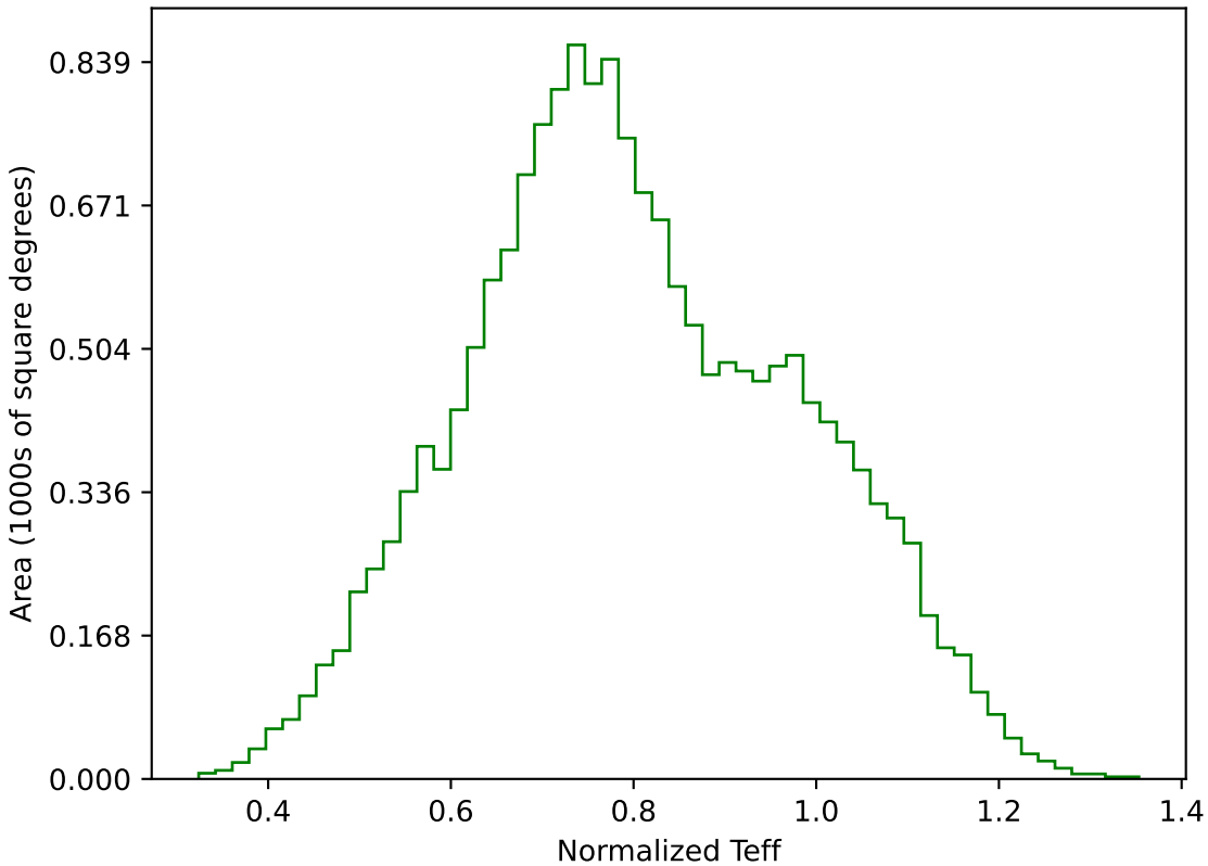
too_elab_r16_d2_griz_v3.4_10yrs WFD g band: Normalized Teff
