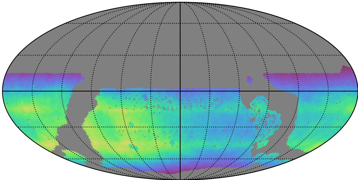
too_elab_r16_d2_griz_v3.4_10yrs WFD all bands: Normalized Teff
