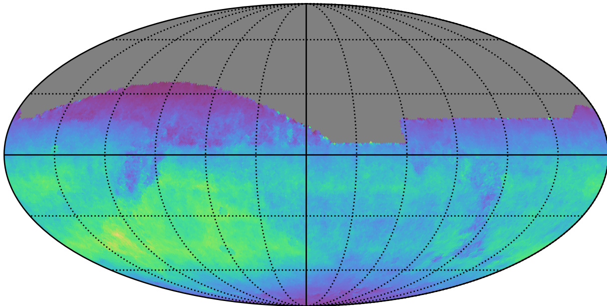
too_elab_r16_d2_griz_v3.4_10yrs All sky z band: Normalized Teff
