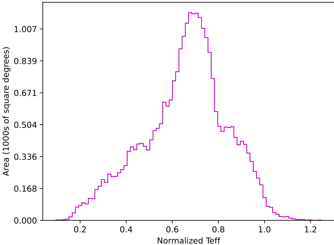
too_elab_r16_d2_griz_v3.4_10yrs All sky z band: Normalized Teff
