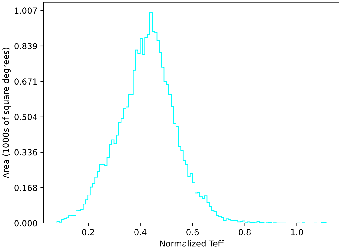
too_elab_r16_d2_griz_v3.4_10yrs All sky u band: Normalized Teff
