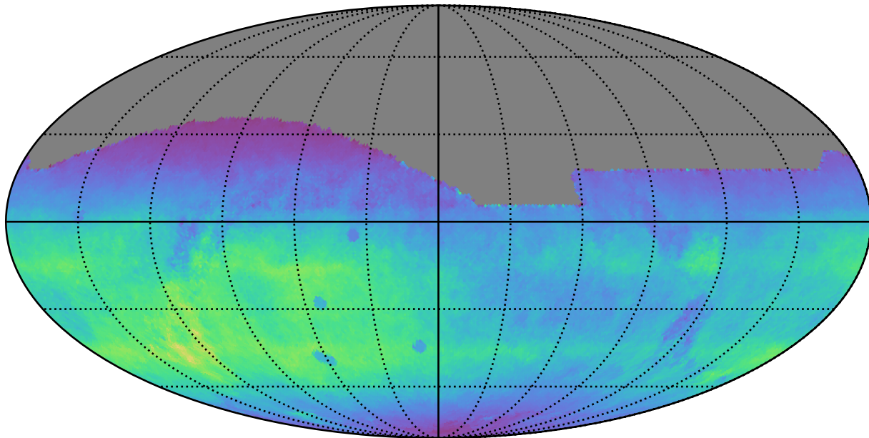
too_elab_r16_d2_griz_v3.4_10yrs All sky r band: Normalized Teff
