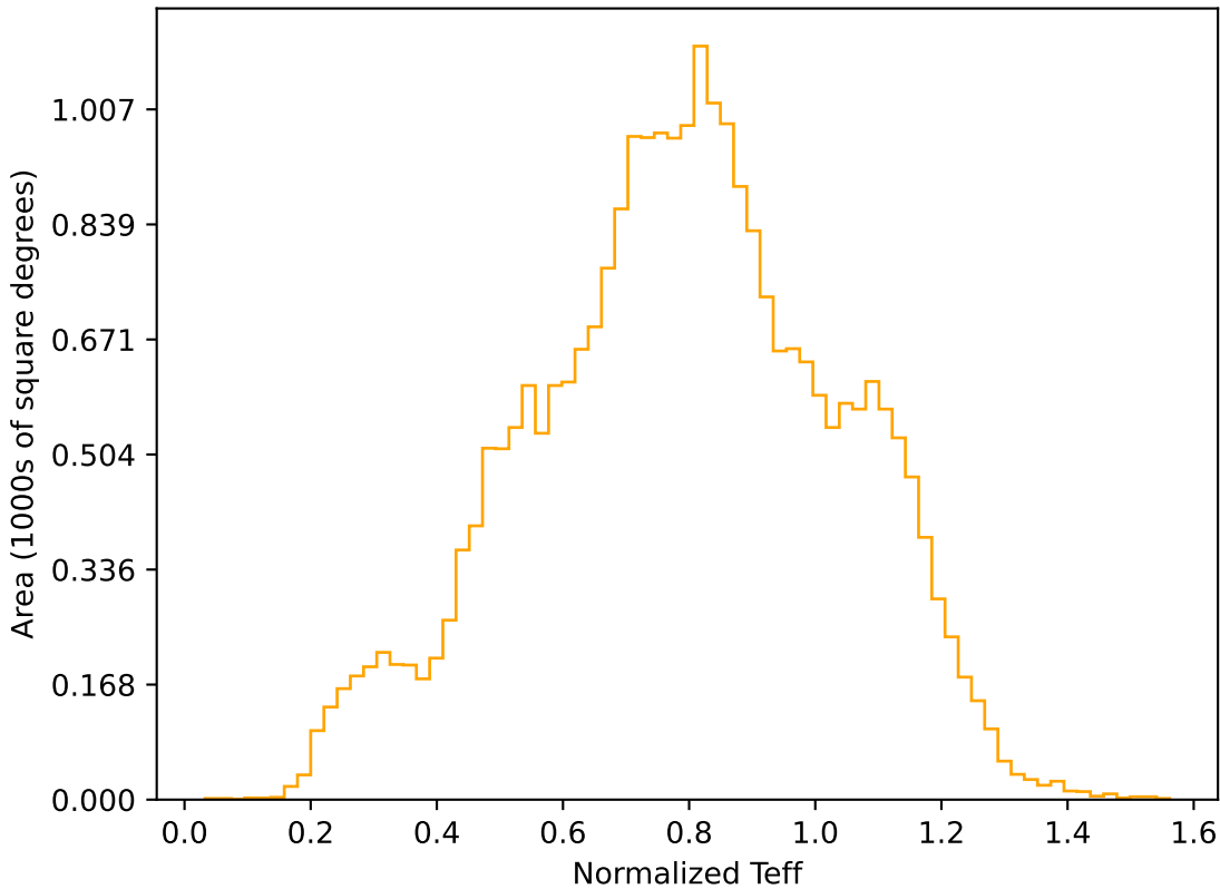
too_elab_r16_d2_griz_v3.4_10yrs All sky r band: Normalized Teff
