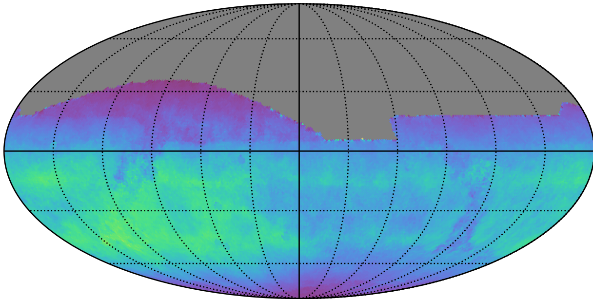
too_elab_r16_d2_griz_v3.4_10yrs All sky i band: Normalized Teff
