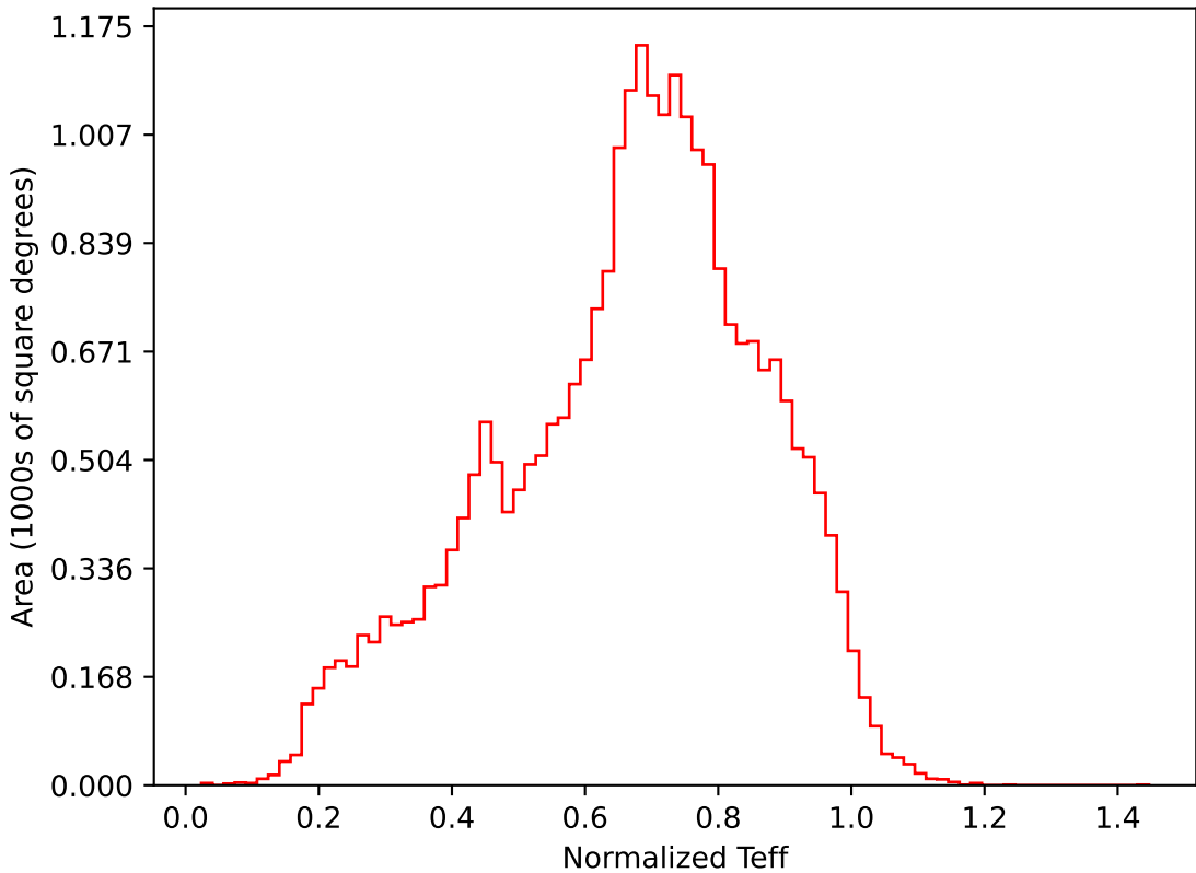
too_elab_r16_d2_griz_v3.4_10yrs All sky i band: Normalized Teff
