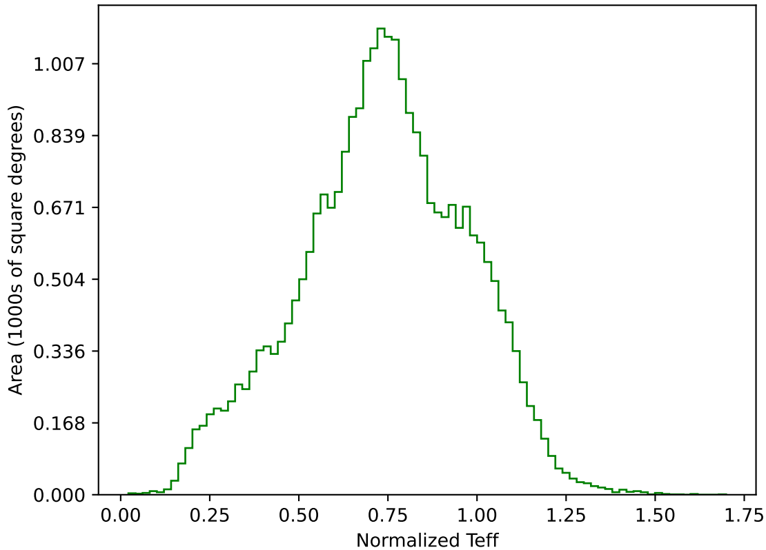
too_elab_r16_d2_griz_v3.4_10yrs All sky g band: Normalized Teff
