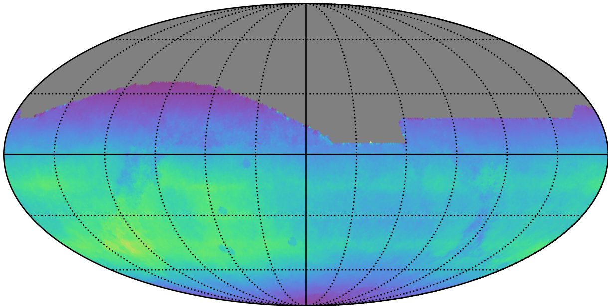
too_elab_r16_d2_griz_v3.4_10yrs All sky all bands: Normalized Teff
