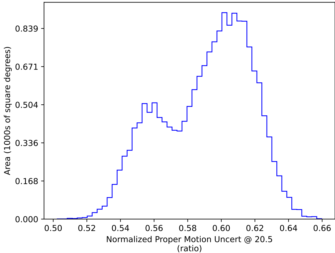
too_elab_r16_d2_griz_v3.4_10yrs WFD: Normalized Proper Motion Uncert @ 20.5
