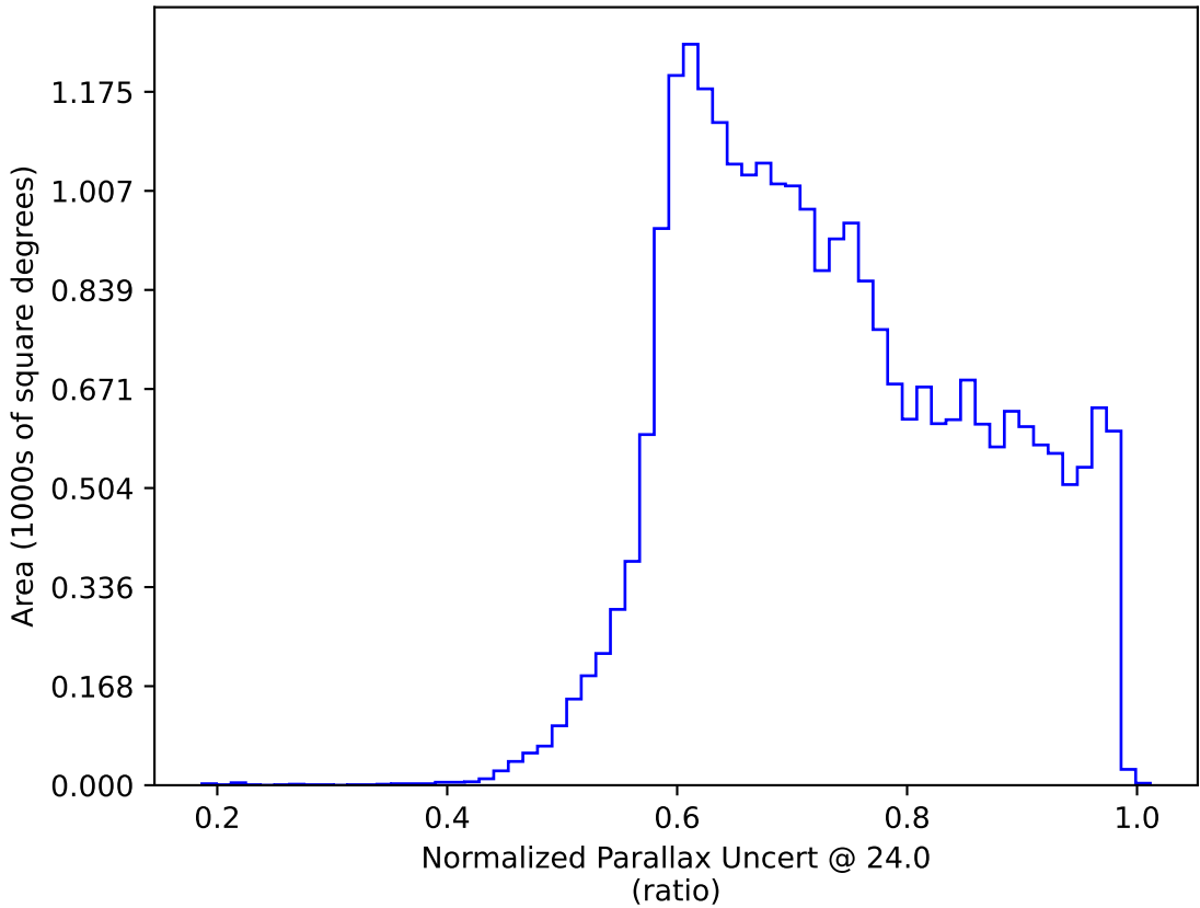
too_elab_r16_d2_griz_v3.4_10yrs All sky: Normalized Parallax Uncert @ 24.0
