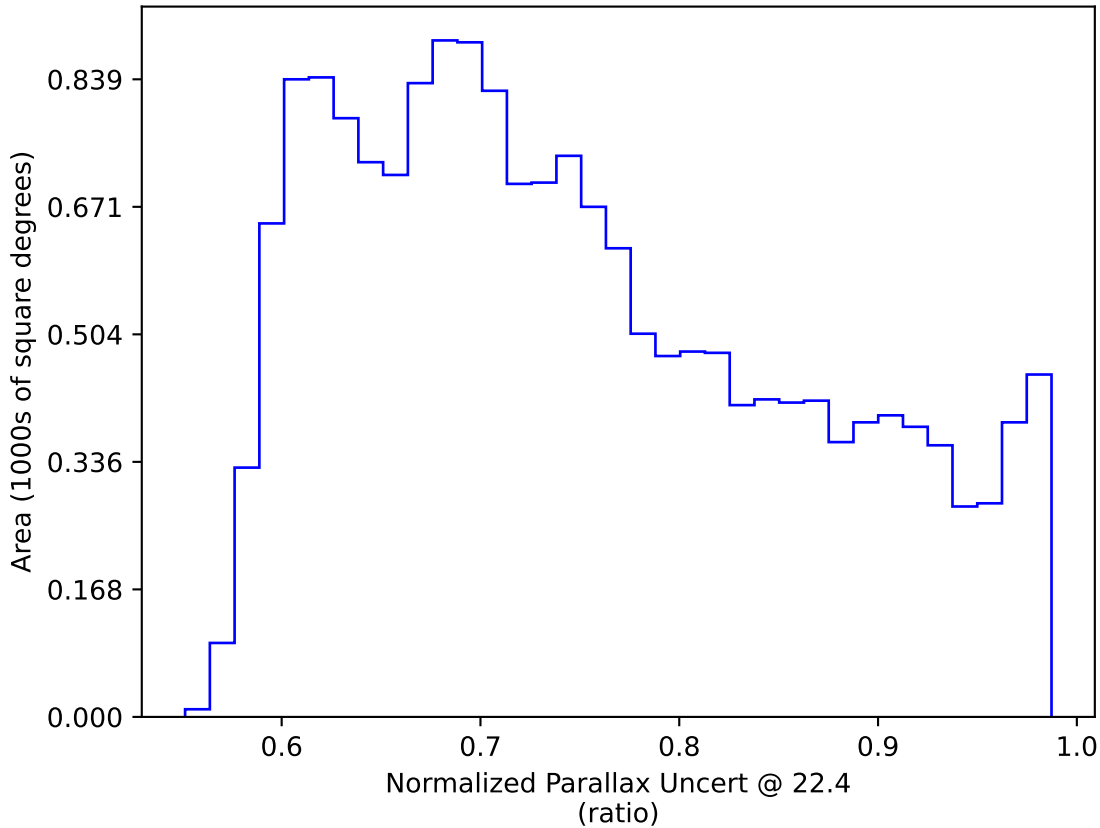
too_elab_r16_d2_griz_v3.4_10yrs WFD: Normalized Parallax Uncert @ 22.4
