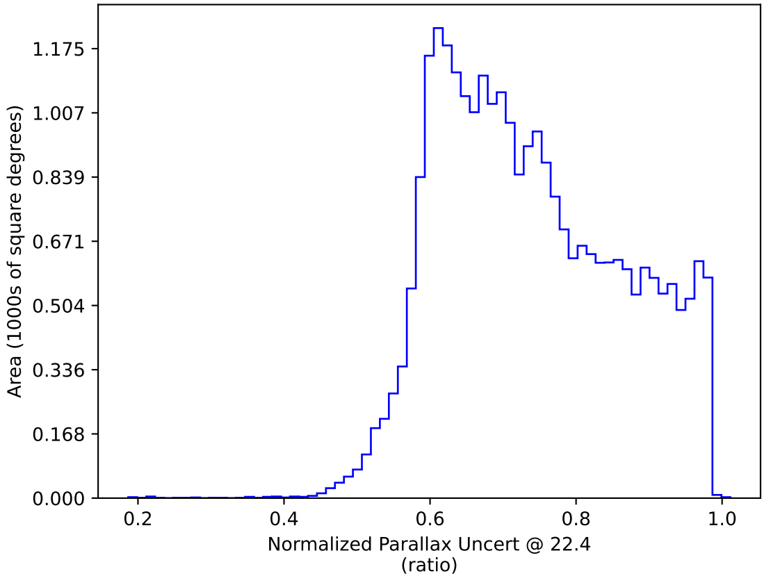
too_elab_r16_d2_griz_v3.4_10yrs All sky: Normalized Parallax Uncert @ 22.4
