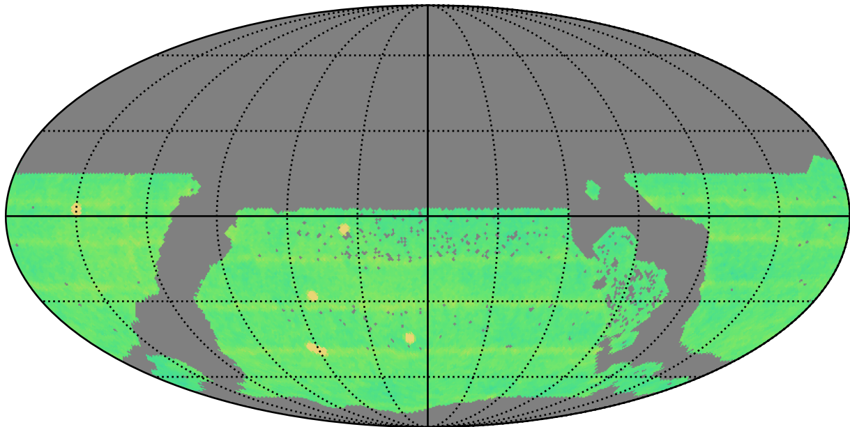
too_elab_r16_d2_griz_v3.4_10yrs WFD all bands: N Unique Nights
