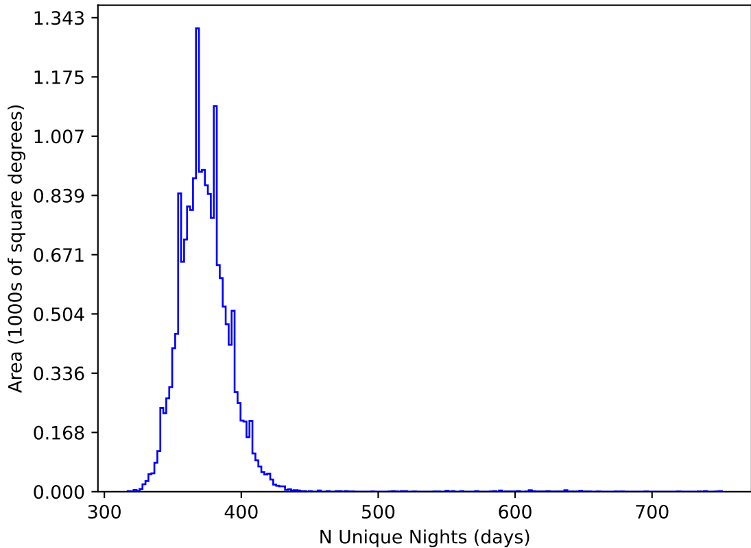
too_elab_r16_d2_griz_v3.4_10yrs WFD all bands: N Unique Nights
