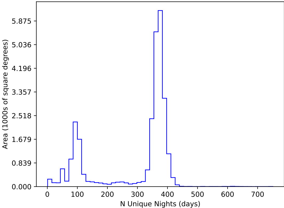
too_elab_r16_d2_griz_v3.4_10yrs All sky all bands: N Unique Nights
