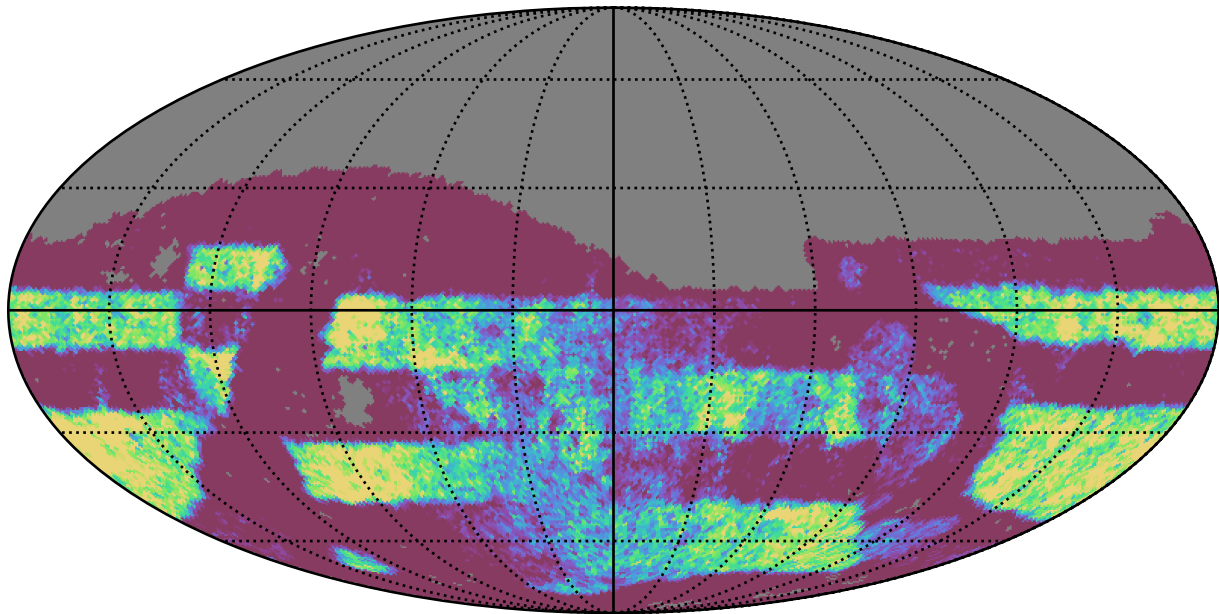
too_elab_r16_d2_griz_v3.4_10yrs Yr 3-4 z band: NVisits
