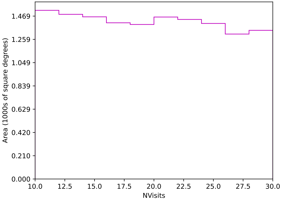
too_elab_r16_d2_griz_v3.4_10yrs Yr 3-4 z band: NVisits
