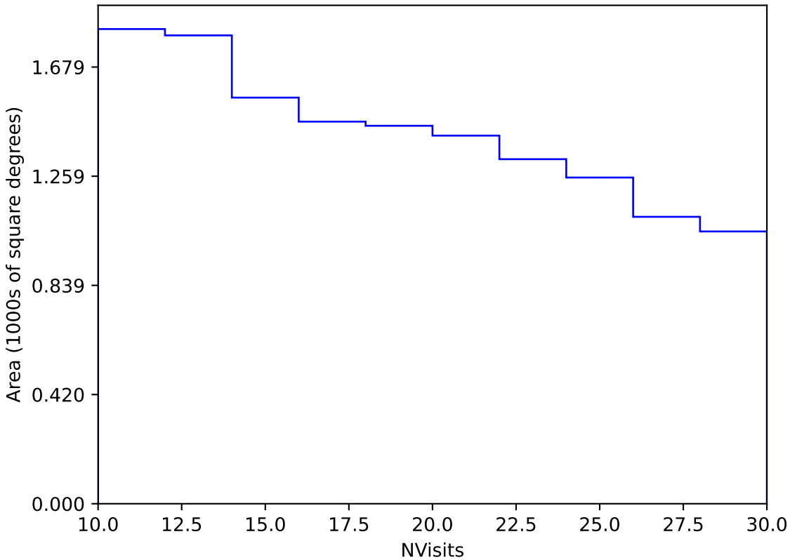
too_elab_r16_d2_griz_v3.4_10yrs Yr 3-4 y band: NVisits
