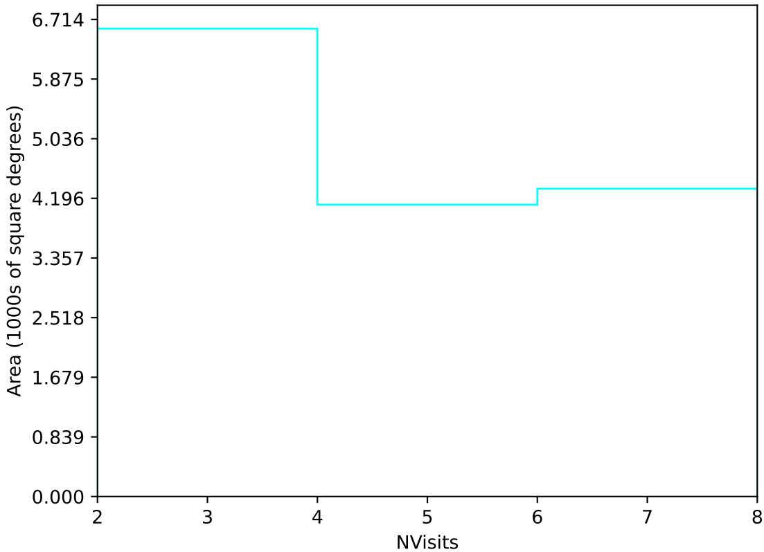
too_elab_r16_d2_griz_v3.4_10yrs Yr 3-4 u band: NVisits
