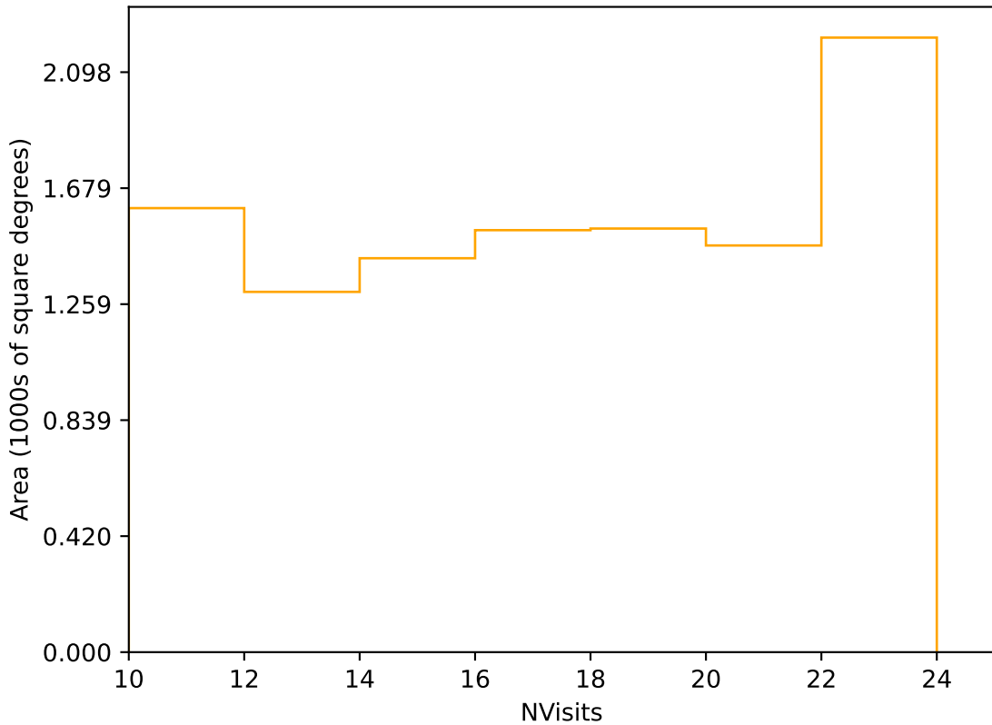
too_elab_r16_d2_griz_v3.4_10yrs Yr 3-4 r band: NVisits
