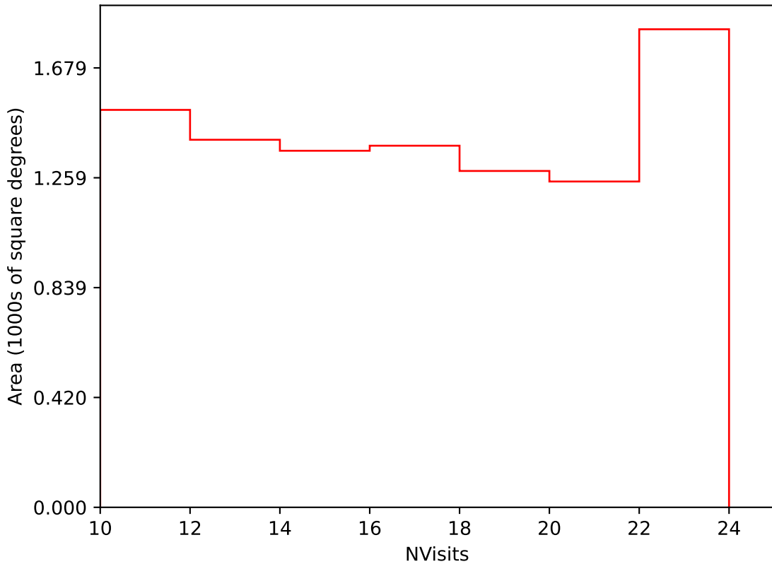
too_elab_r16_d2_griz_v3.4_10yrs Yr 3-4 i band: NVisits
