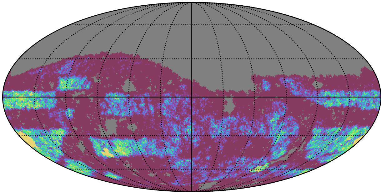
too_elab_r16_d2_griz_v3.4_10yrs Yr 3-4 g band: NVisits
