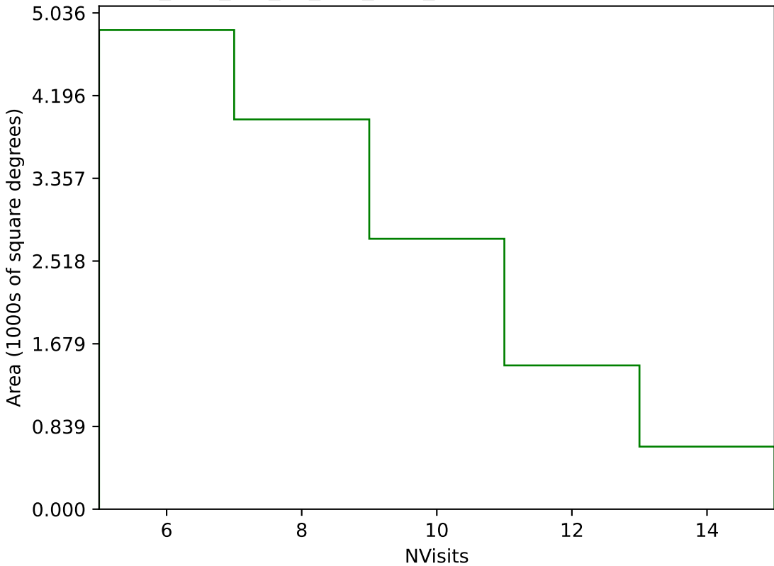
too_elab_r16_d2_griz_v3.4_10yrs Yr 3-4 g band: NVisits
