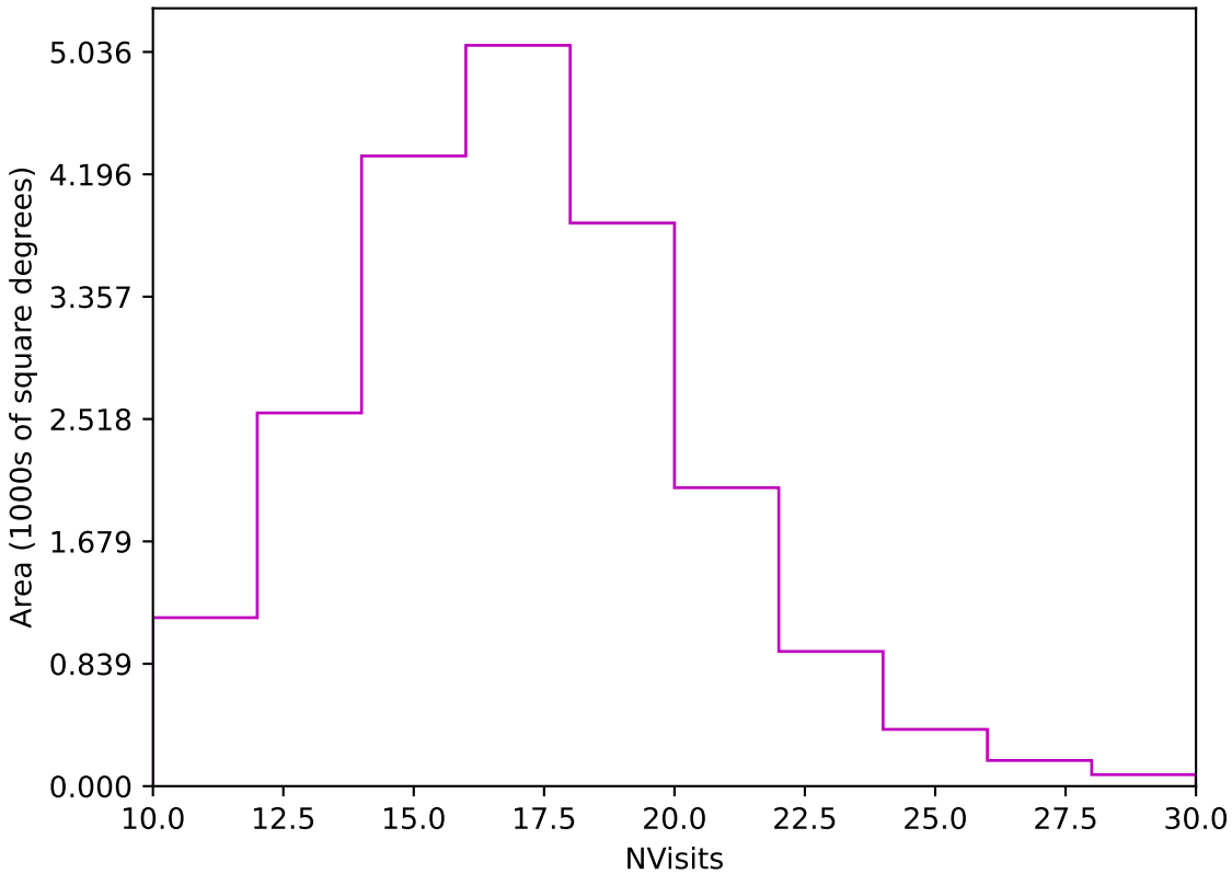
too_elab_r16_d2_griz_v3.4_10yrs Yr 1 z band: NVisits
