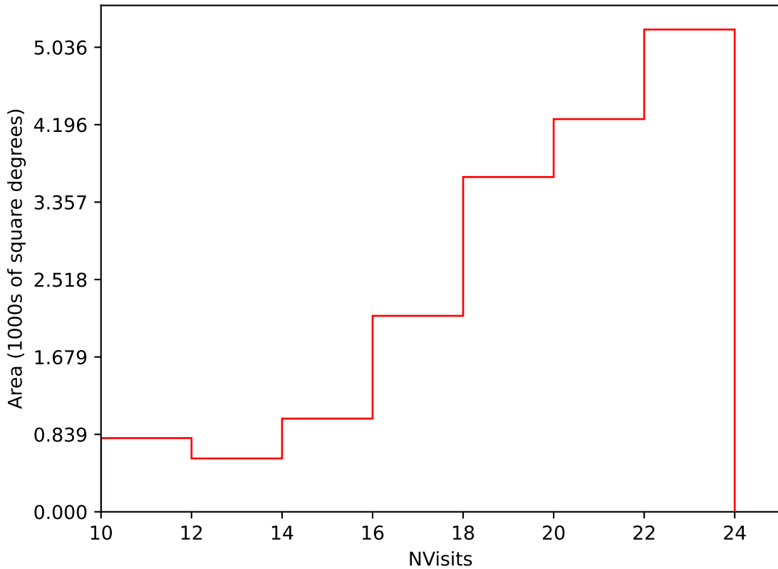
too_elab_r16_d2_griz_v3.4_10yrs Yr 1 i band: NVisits
