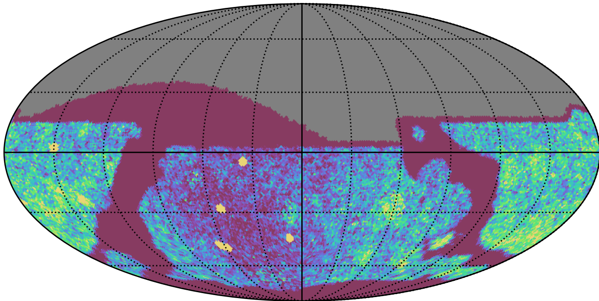
too_elab_r16_d2_griz_v3.4_10yrs Yr 1 all bands: NVisits
