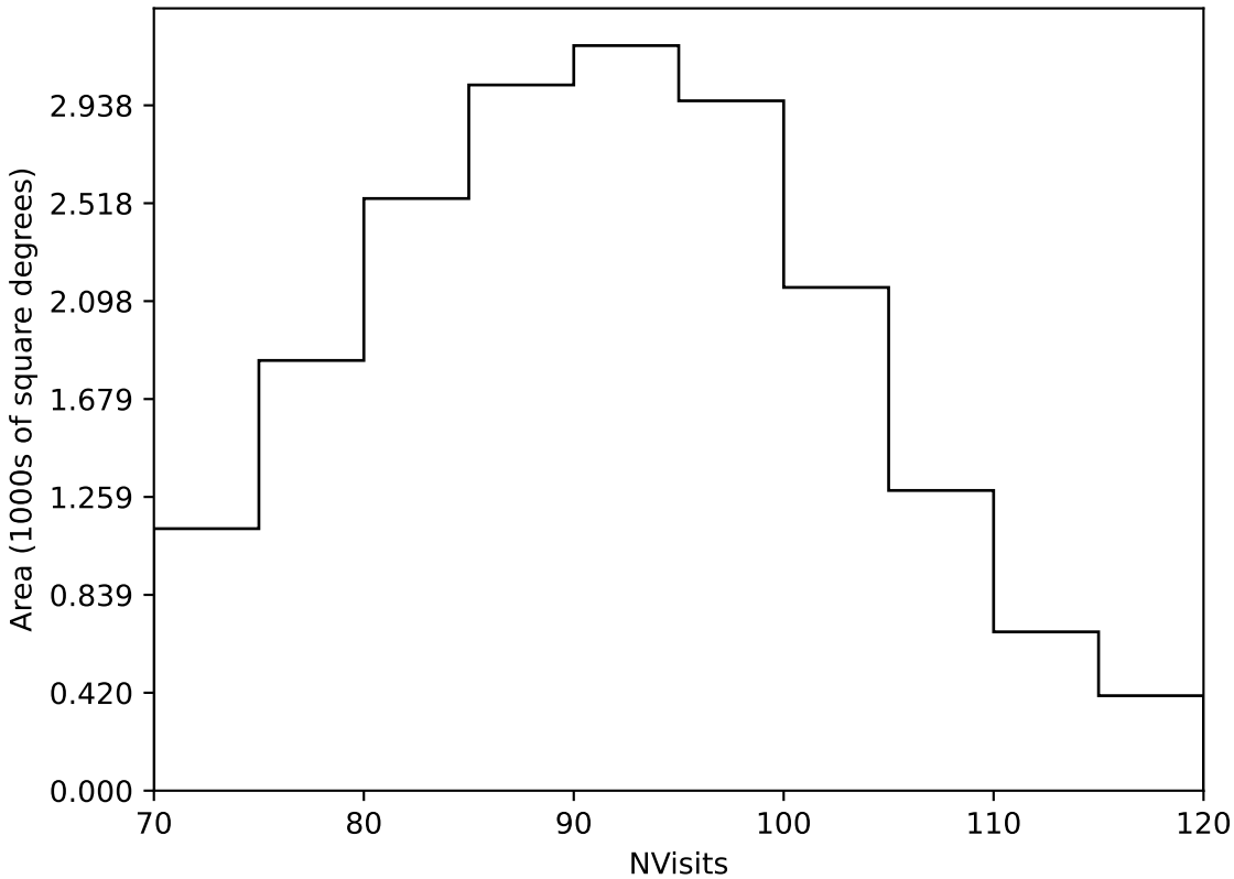
too_elab_r16_d2_griz_v3.4_10yrs Yr 1 all bands: NVisits
