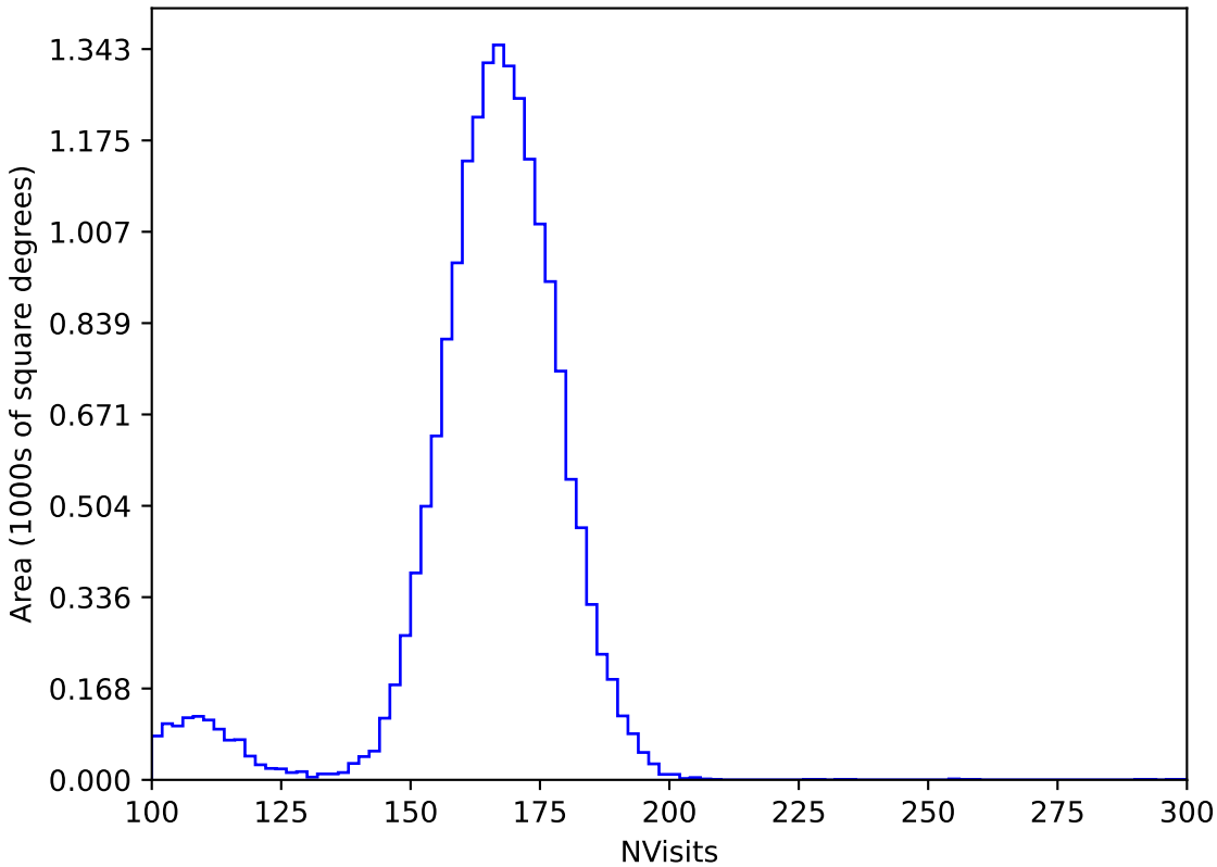
too_elab_r16_d2_griz_v3.4_10yrs WFD y band: NVisits
