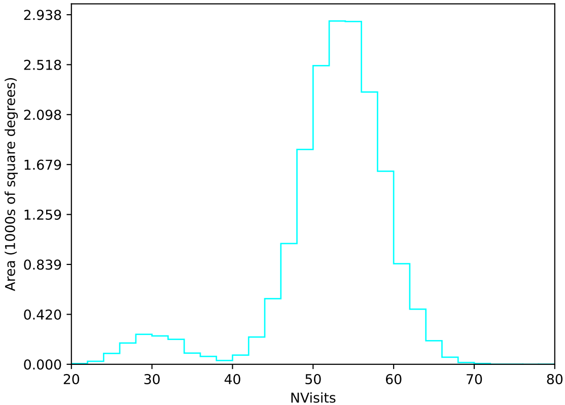
too_elab_r16_d2_griz_v3.4_10yrs WFD u band: NVisits
