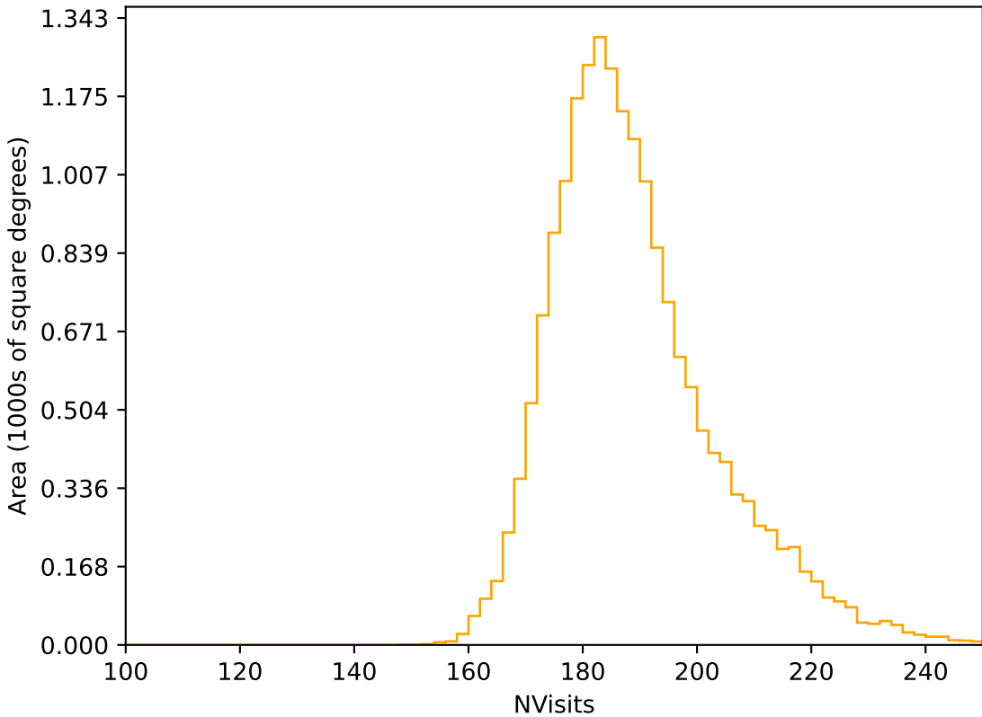
too_elab_r16_d2_griz_v3.4_10yrs WFD r band: NVisits
