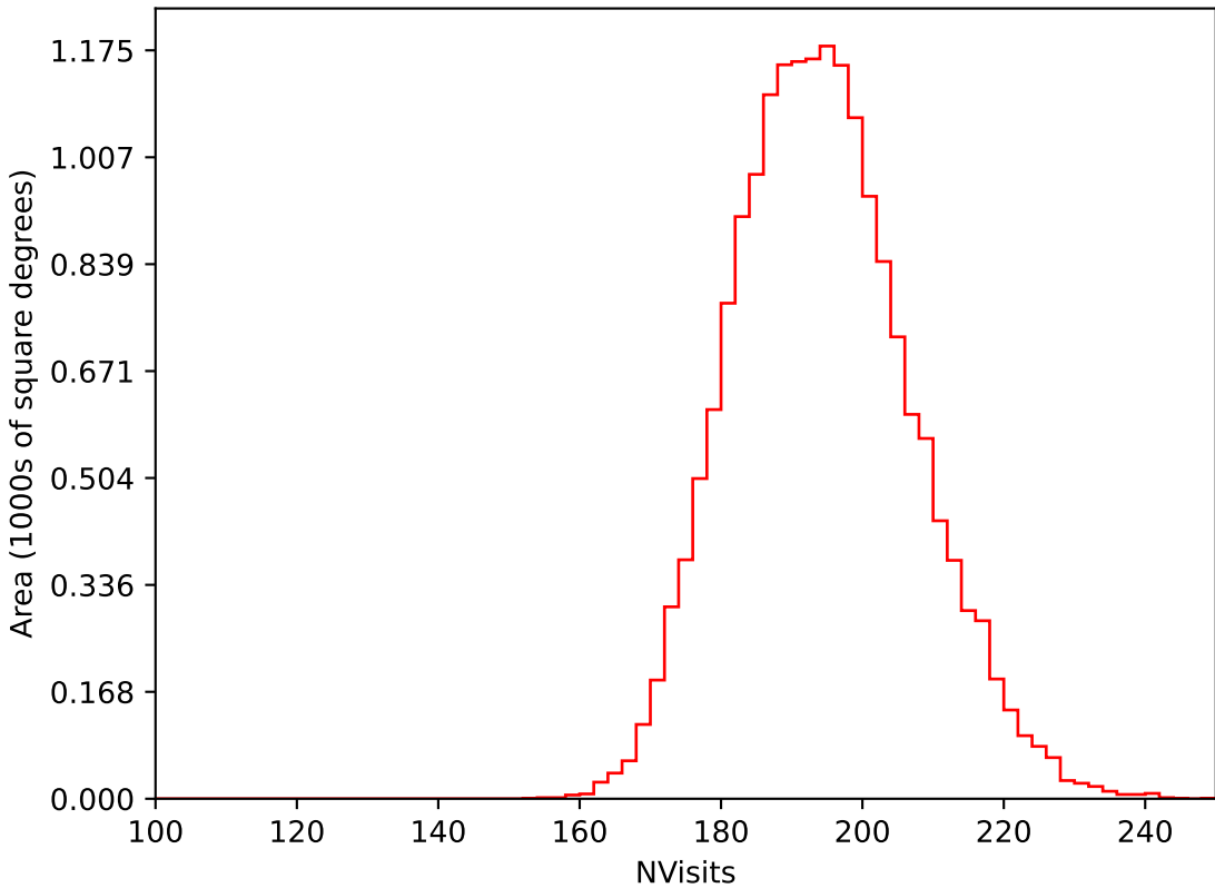
too_elab_r16_d2_griz_v3.4_10yrs WFD i band: NVisits
