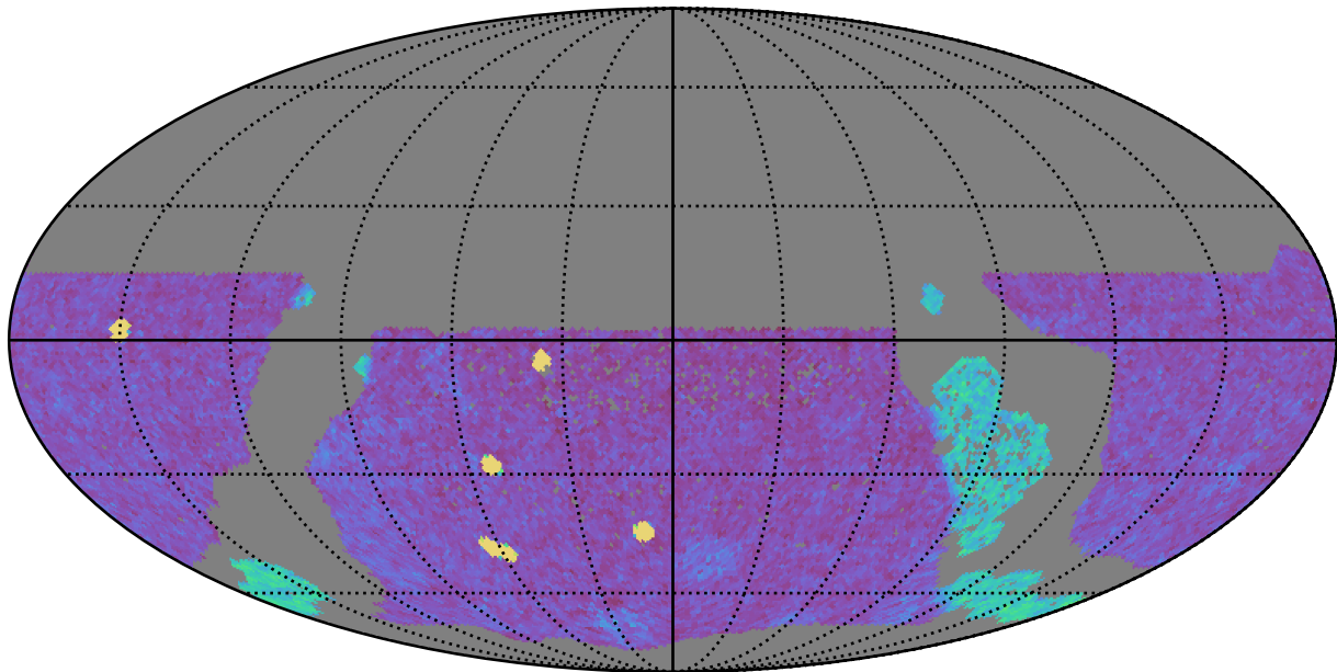
too_elab_r16_d2_griz_v3.4_10yrs WFD g band: NVisits
