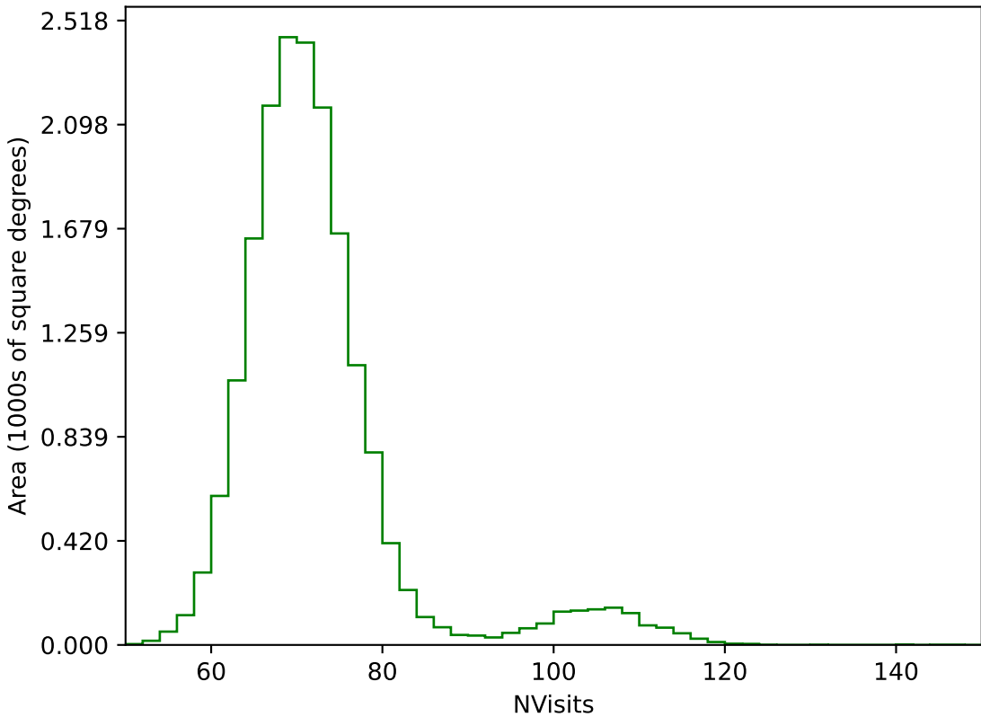
too_elab_r16_d2_griz_v3.4_10yrs WFD g band: NVisits
